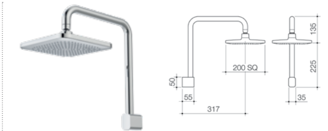
Luna Contemporary Fixed Overhead Shower WELS 4 star rated, 6-7.5L/min 90391C4E
