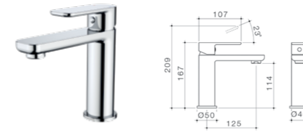
Luna Standard Basin Mixer WELS 5 star rated, 6L/min 68181C5A
