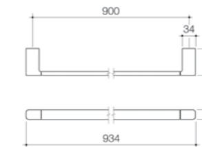
Luna Contemporary Single Towel Rail 930mm 99613C
