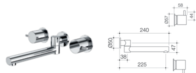
Luna Contemporary Lever Laundry Tap Set WELS 4 star rated, 6-7.5L/min 90331C4A
