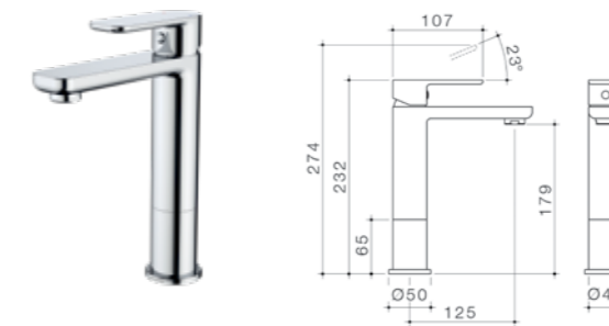
Luna Mid Basin Mixer WELS 5 star rated, 6L/min 68182C5A
