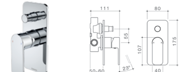
Luna Bath/Shower Mixer With Diverter With Diverter 68185C
