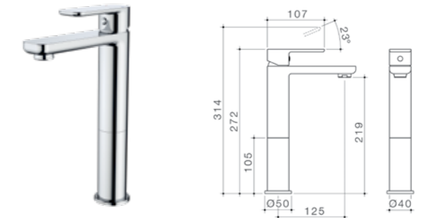
Luna Tower Basin Mixer WELS 5 star rated, 6L/min 68183C5A
