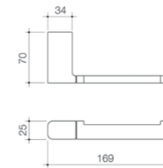
Luna Contemporary Toilet Roll Holder 99607C
