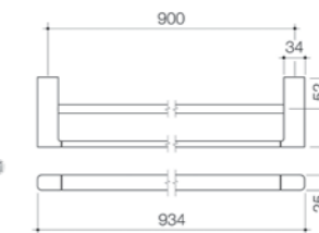
Luna Contemporary Double Towel Rail 930mm 99615C
