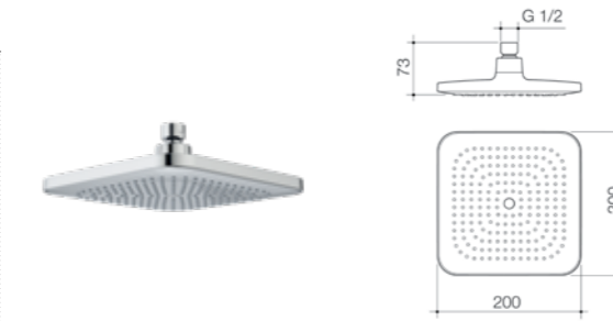
Luna Contemporary Overhead Shower Head Only WELS 4 star rated, 6-7.5L/min 90386C4E
