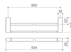
Luna Contemporary Double Towel Rail 630mm 99614C
