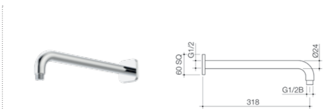
Luna Contemporary Ceiling Shower Arm Right angle 90390C
