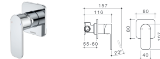
Luna Bath/Shower Mixer Without Diverter 68184C
