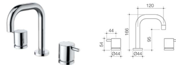
Luna Contemporary Lever Basin Tap Set WELS 5 star rated, 4.5-6L/min 90334C5A
