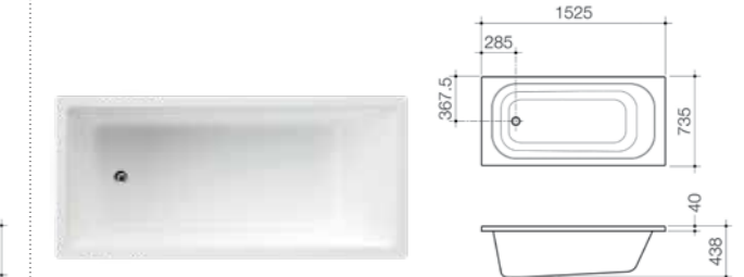
Luna Island Bath
