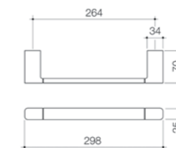
Luna Contemporary Hand Towel Rail 99611C
