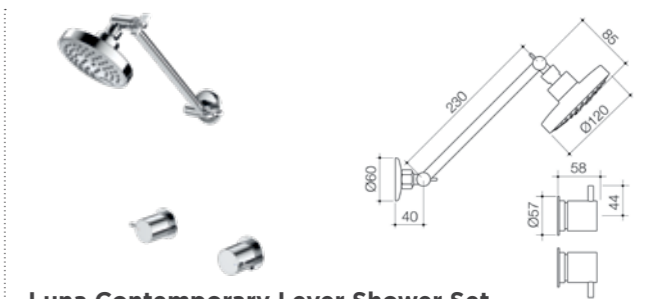
Luna Contemporary Lever Shower Set WELS 3 star rated, 7.5-9L/min 90332C3A
