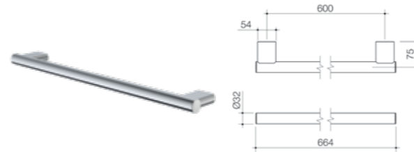
Opal Support Rail 600mm Straight 687377C
