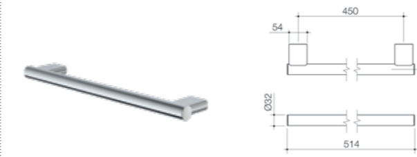
Opal Support Rail 450mm Straight 687376C
