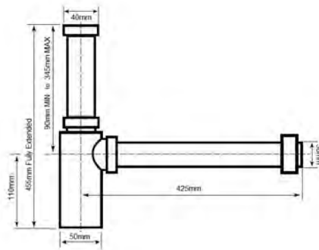
VERTICAL EXTENSION PIPE FOR ROUND BOTTLE P-TRAP
