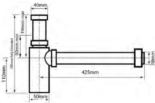
AURORA ADJUSTABLE BOTTLE P-TRAP
